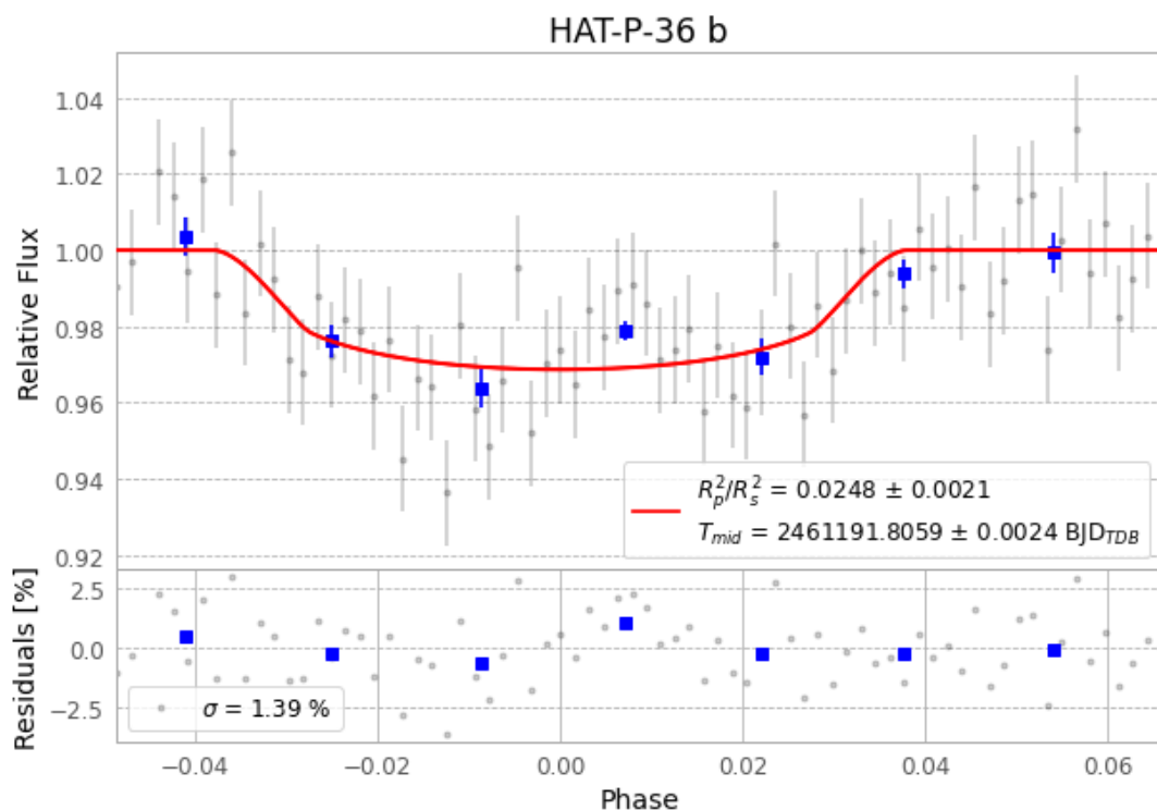
Figure 1 — FinalLightCurve_HAT-P-36 b_2026-05-30.png (SHA-256 2c64b8bc98a00324...)
