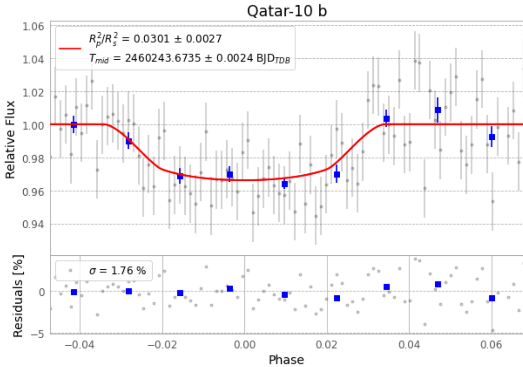
Figure 1 — FinalLightCurve_Qatar-10 b_2023-10-25.png (SHA-256 e6d029be4baece25...)
