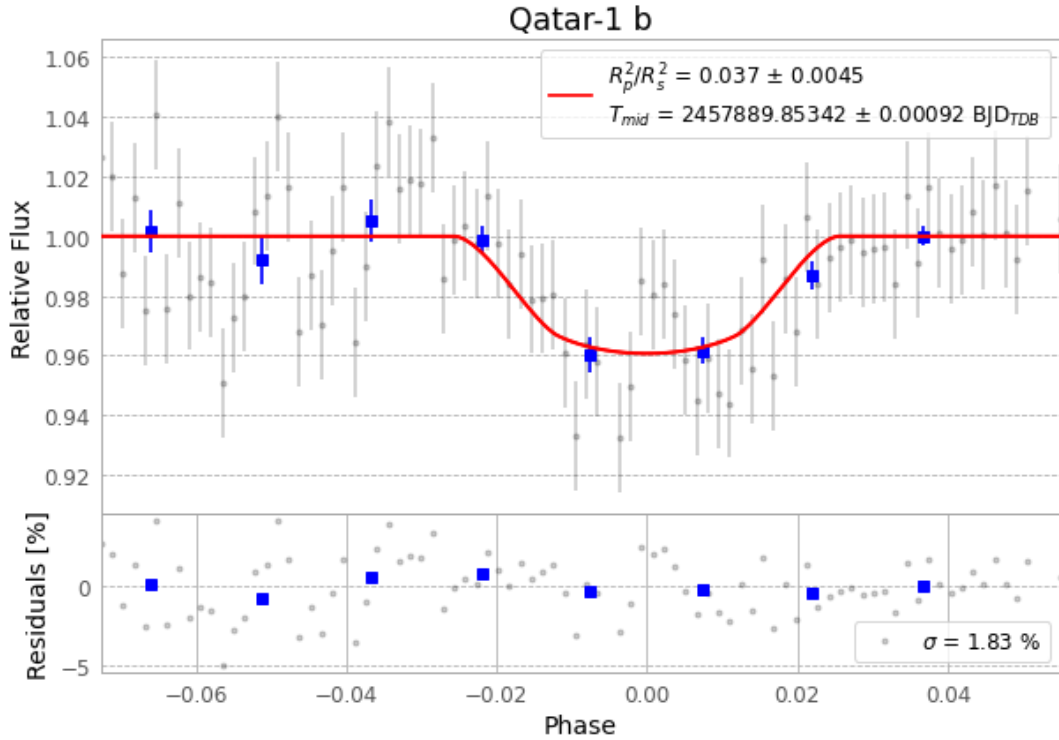
Figure 1 — FinalLightCurve_Qatar-1 b_2017-05-15.png (SHA-256 fc4d2ba12336a678...)
