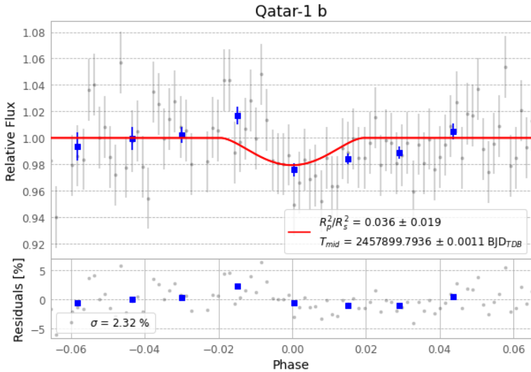
Figure 1 — FinalLightCurve_Qatar-1 b_2017-05-25.png (SHA-256 2a8741732af749ea...)
