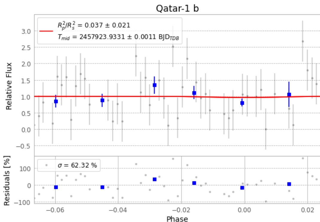
Figure 1 — FinalLightCurve_Qatar-1 b_2017-06-19.png (SHA-256 76e2aa2318ae9439...)
