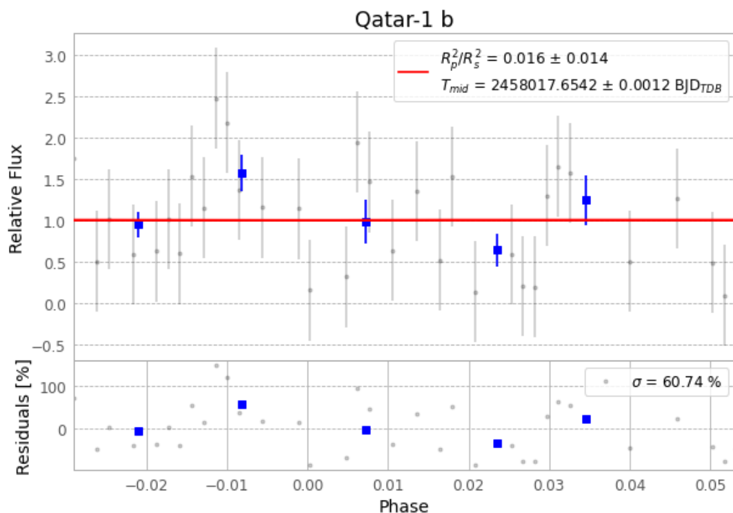
Figure 1 — FinalLightCurve_Qatar-1 b_2017-09-20.png (SHA-256 79d59c51542dc65e...)
