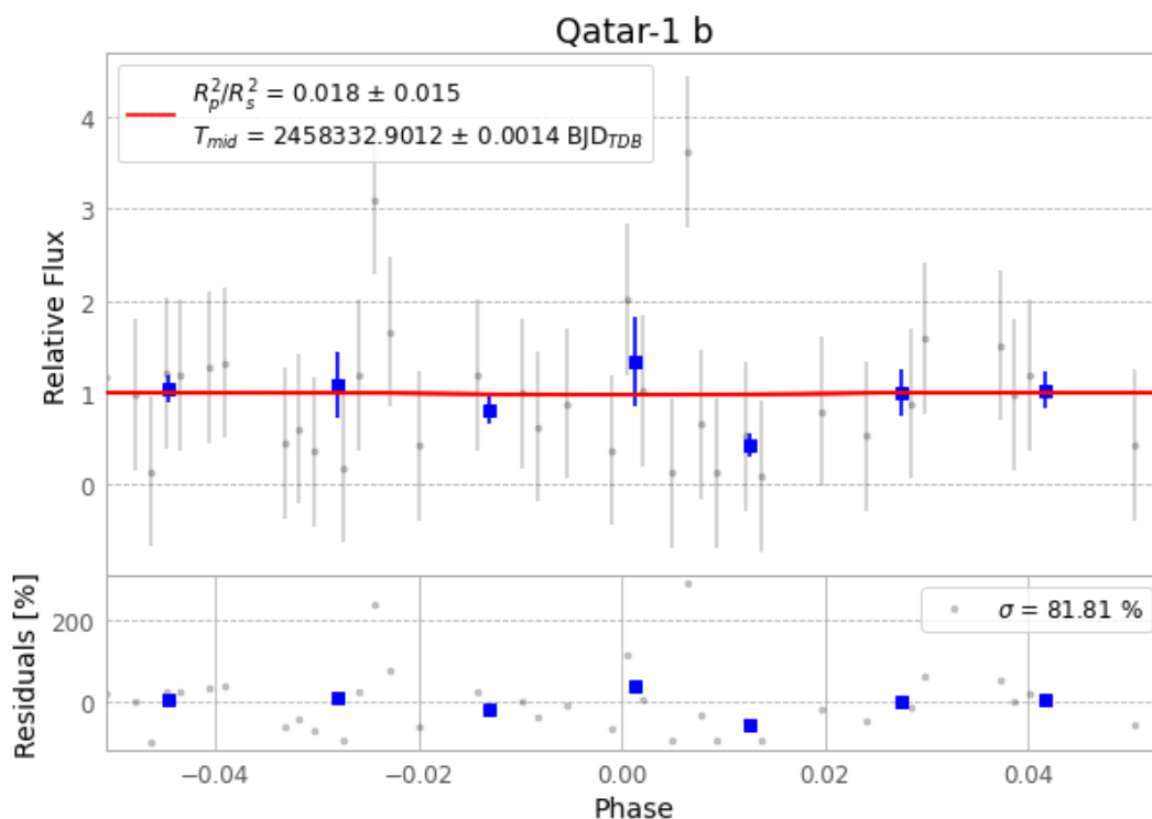
Figure 1 — FinalLightCurve_Qatar-1 b_2018-08-02.png (SHA-256 adec933c329cbafe...)
