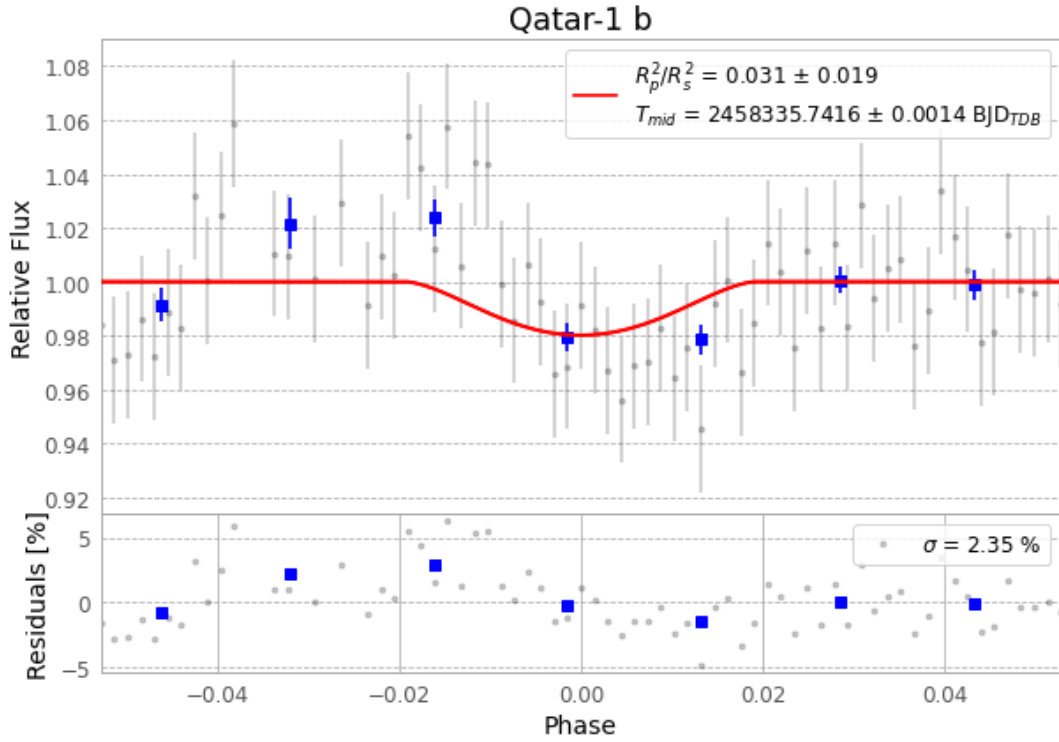
Figure 1 — FinalLightCurve_Qatar-1 b_2018-08-04.png (SHA-256 897cb5a078392c23...)
