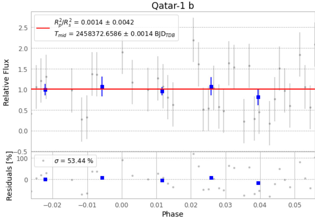
Figure 1 — FinalLightCurve_Qatar-1 b_2018-09-10.png (SHA-256 f061d85a20af6021...)
