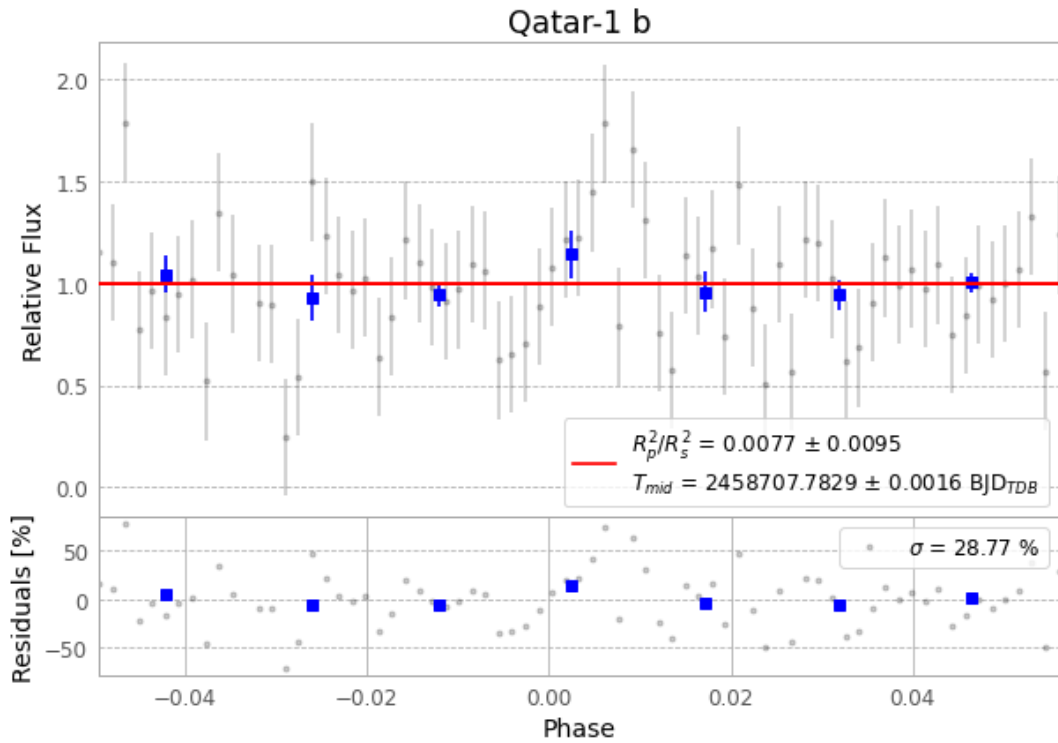
Figure 1 — FinalLightCurve_Qatar-1 b_2019-08-11.png (SHA-256 2bcb841188c36829...)
