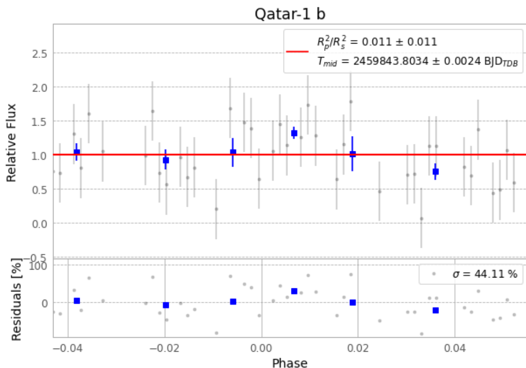
Figure 1 — FinalLightCurve_Qatar-1 b_2022-09-20.png (SHA-256 ee0ebc2e27ced842...)
