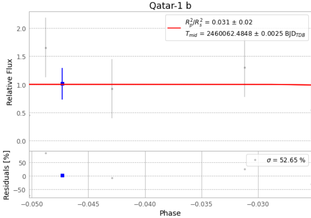
Figure 1 — FinalLightCurve_Qatar-1 b_2023-04-29.png (SHA-256 e90e93a676bd01f6...)
