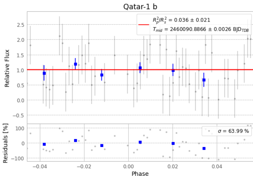
Figure 1 — FinalLightCurve_Qatar-1 b_2023-05-26.png (SHA-256 e09b1363fe29e89e...)
