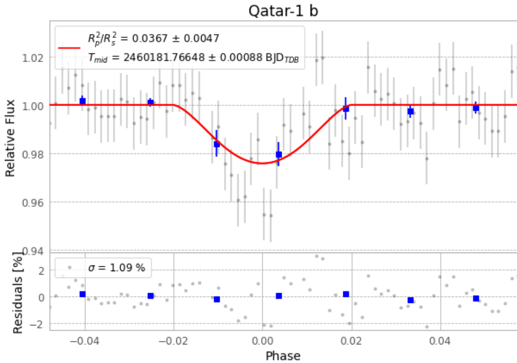
Figure 1 — FinalLightCurve_Qatar-1 b_2023-08-24.png (SHA-256 c7023adff7ad05b4...)
