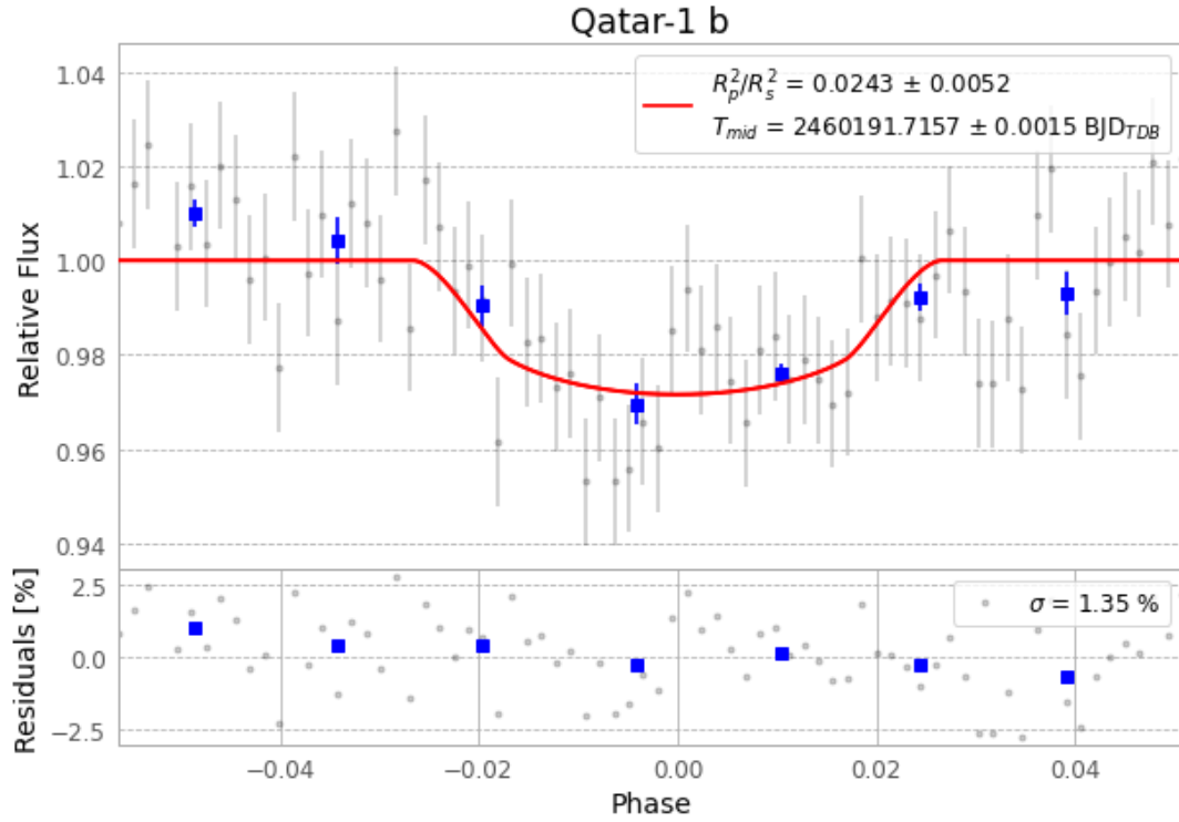
Figure 1 — FinalLightCurve_Qatar-1 b_2023-09-03.png (SHA-256 e39869643f5d6652...)
