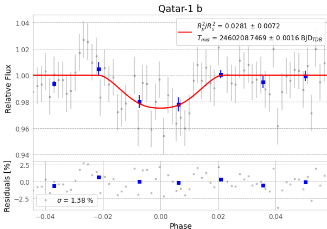
Figure 1 — FinalLightCurve_Qatar-1 b_2023-09-20.png (SHA-256 98a4721c687540c8...)
