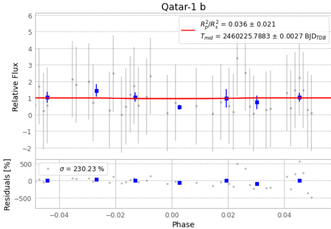
Figure 1 — FinalLightCurve_Qatar-1 b_2023-10-07.png (SHA-256 8ea7c34a4aad7595...)
