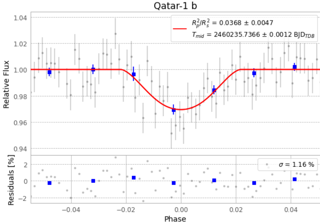
Figure 1 — FinalLightCurve_Qatar-1 b_2023-10-17.png (SHA-256 b9af751c8fb128c5...)
