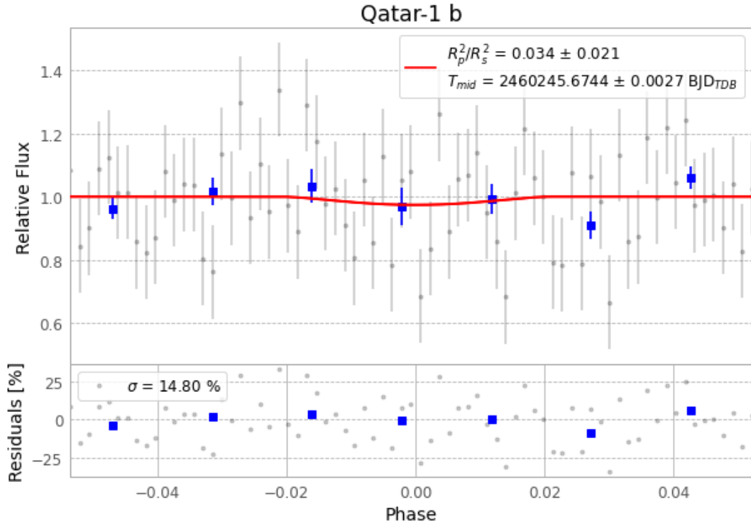
Figure 1 — FinalLightCurve_Qatar-1 b_2023-10-27.png (SHA-256 810165ffd91e9f7e...)
