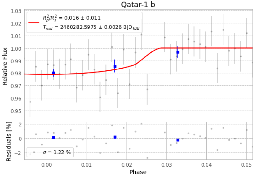
Figure 1 — FinalLightCurve_Qatar-1 b_2023-12-03.png (SHA-256 f4fdf0f740f188e5...)
