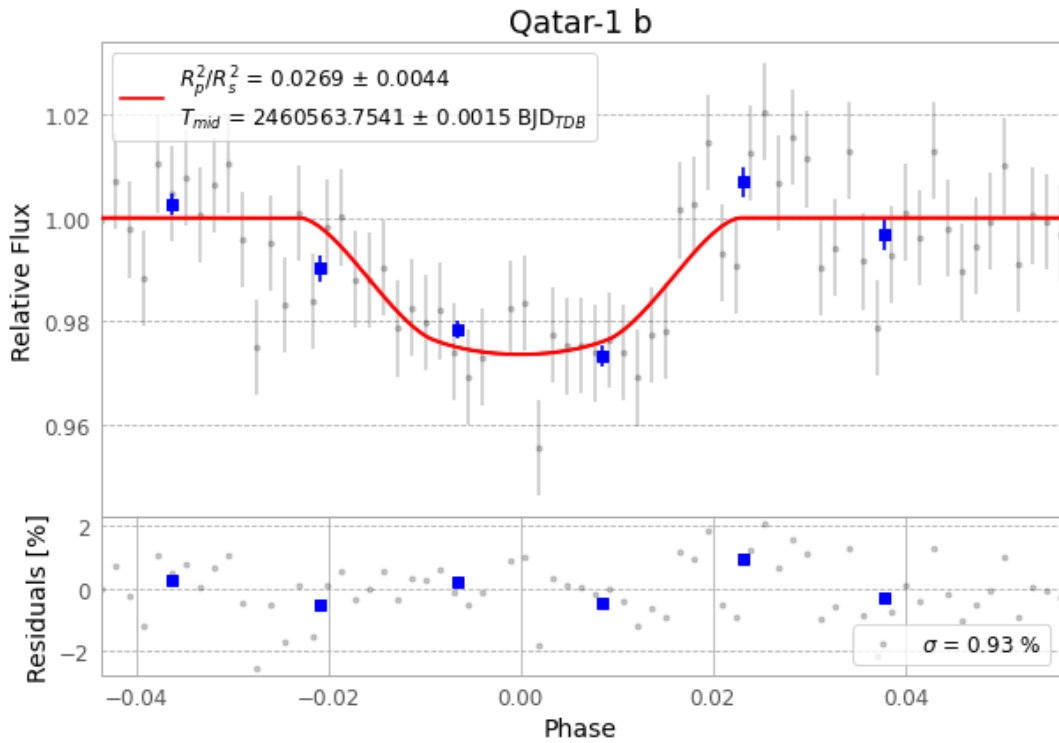
Figure 1 — FinalLightCurve_Qatar-1 b_2024-09-09.png (SHA-256 d6a44501f722cdfb...)
