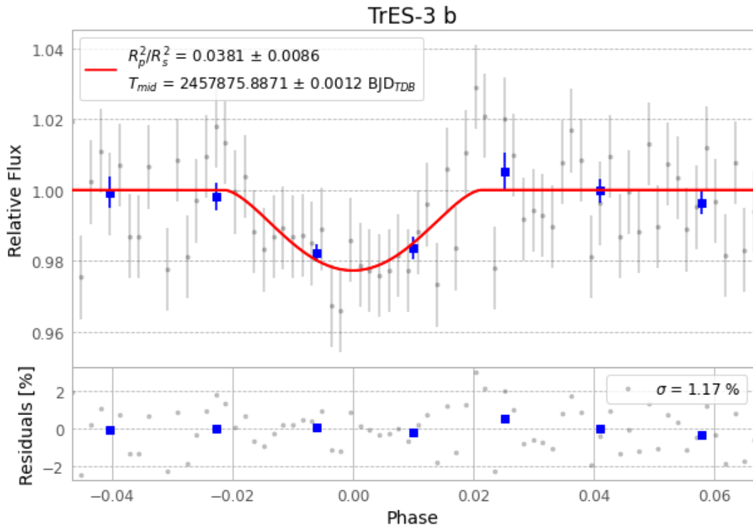
Figure 1 — FinalLightCurve_TrES-3 b_2017-05-02.png (SHA-256 0d7679462f274193...)
