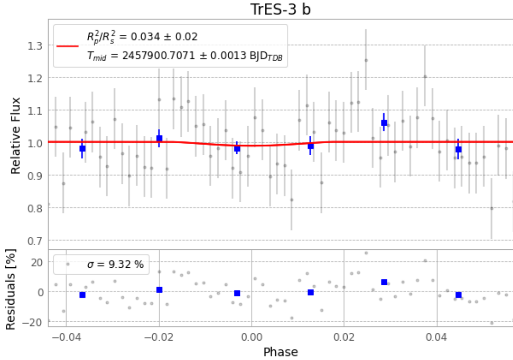
Figure 1 — FinalLightCurve_TrES-3 b_2017-05-26.png (SHA-256 0715bf02b8e0f58f...)
