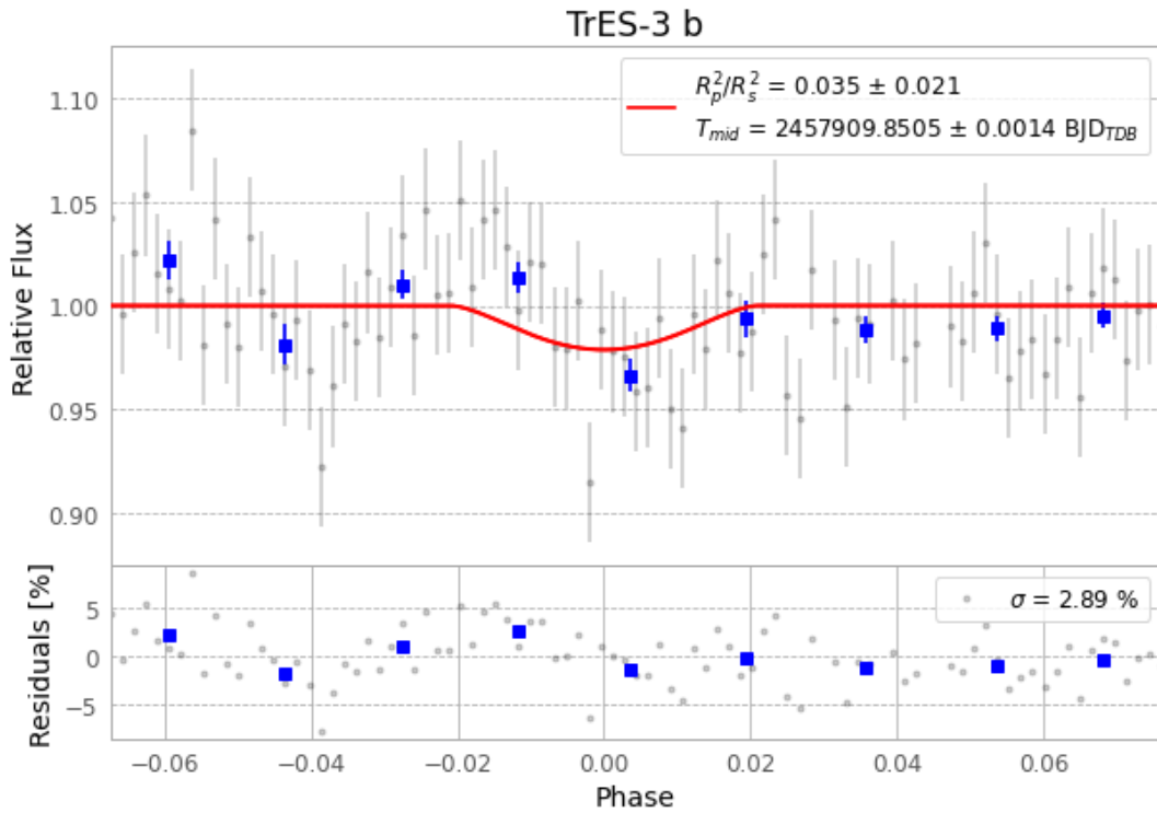
Figure 1 — FinalLightCurve_TrES-3 b_2017-06-04.png (SHA-256 851ff0ba27bc923b...)
