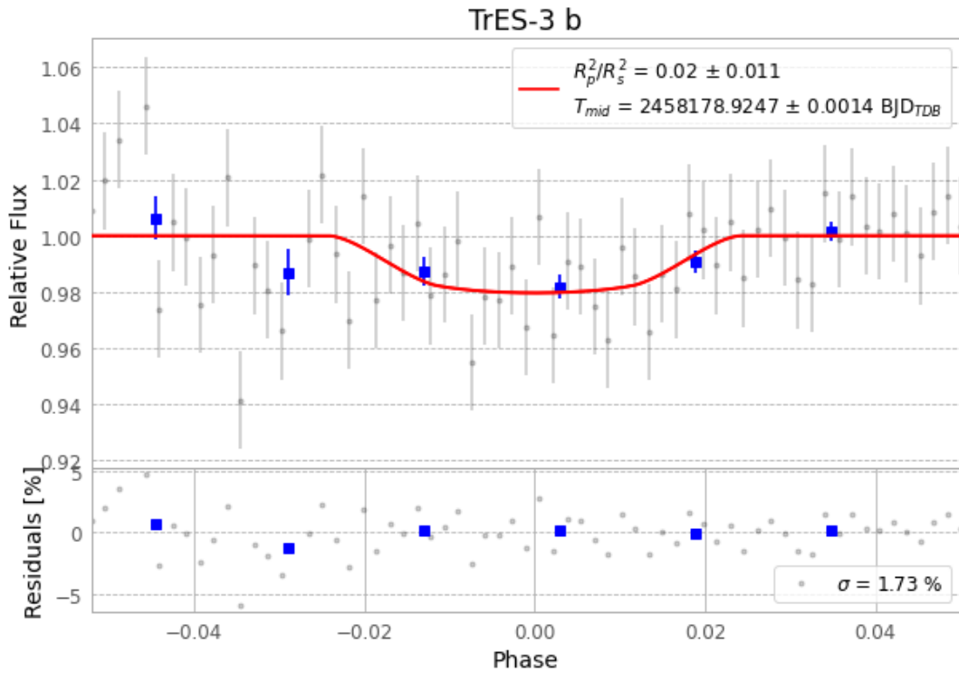
Figure 1 — FinalLightCurve_TrES-3 b_2018-03-01.png (SHA-256 aa6965ed8feb65d3...)
