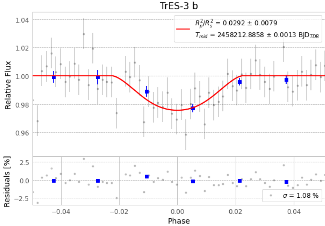
Figure 1 — FinalLightCurve_TrES-3 b_2018-04-04.png (SHA-256 c1aea6adbf750f2a...)
