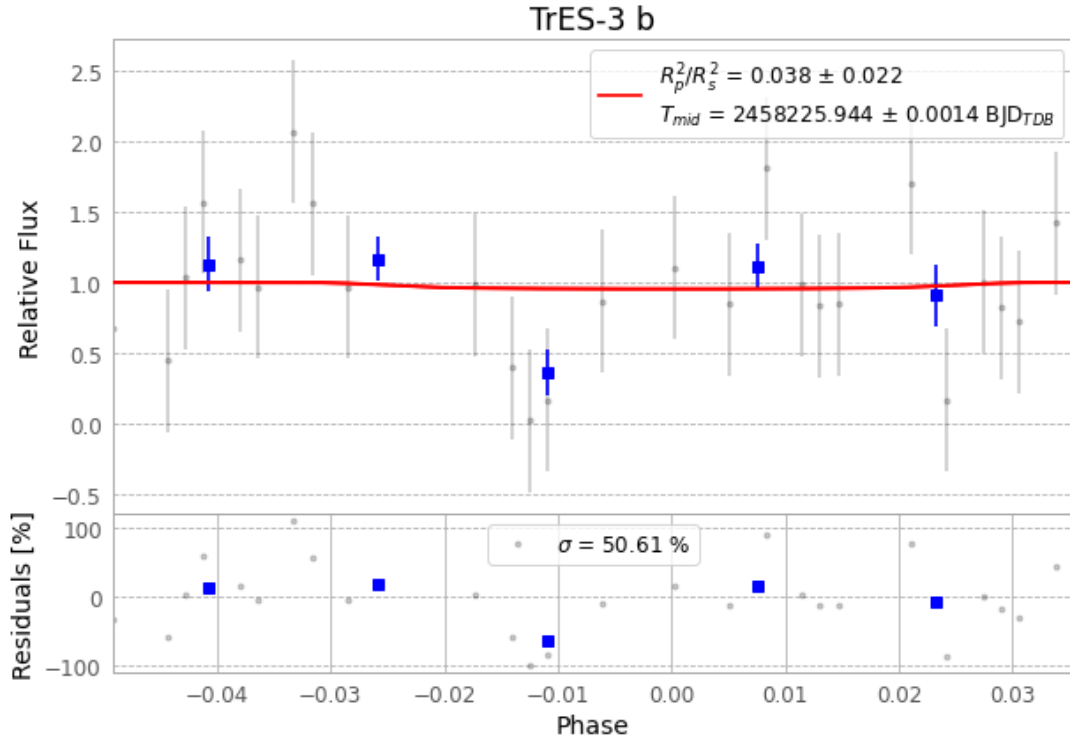
Figure 1 — FinalLightCurve_TrES-3 b_2018-04-17.png (SHA-256 5997822f7c60018a...)
