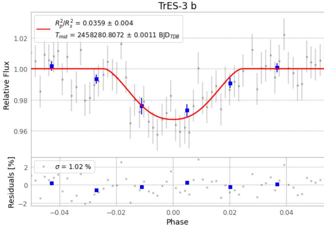
Figure 1 — FinalLightCurve_TrES-3 b_2018-06-10.png (SHA-256 eb8a3df4982a9384...)
