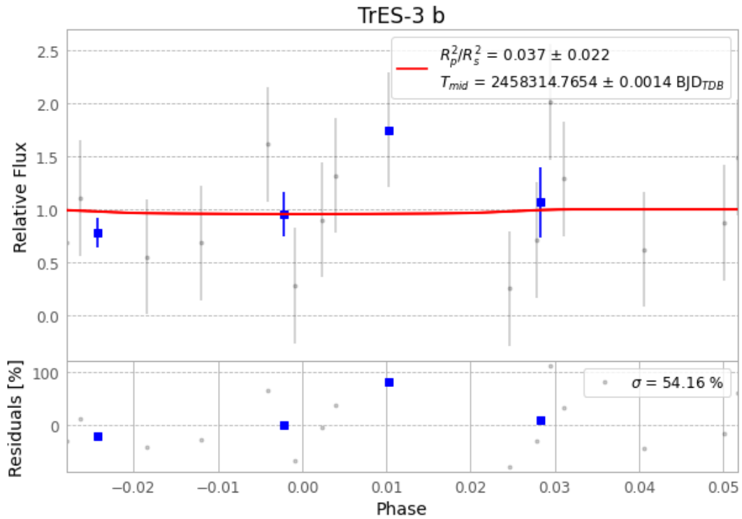
Figure 1 — FinalLightCurve_TrES-3 b_2018-07-14.png (SHA-256 c4862b5757e56d5f...)
