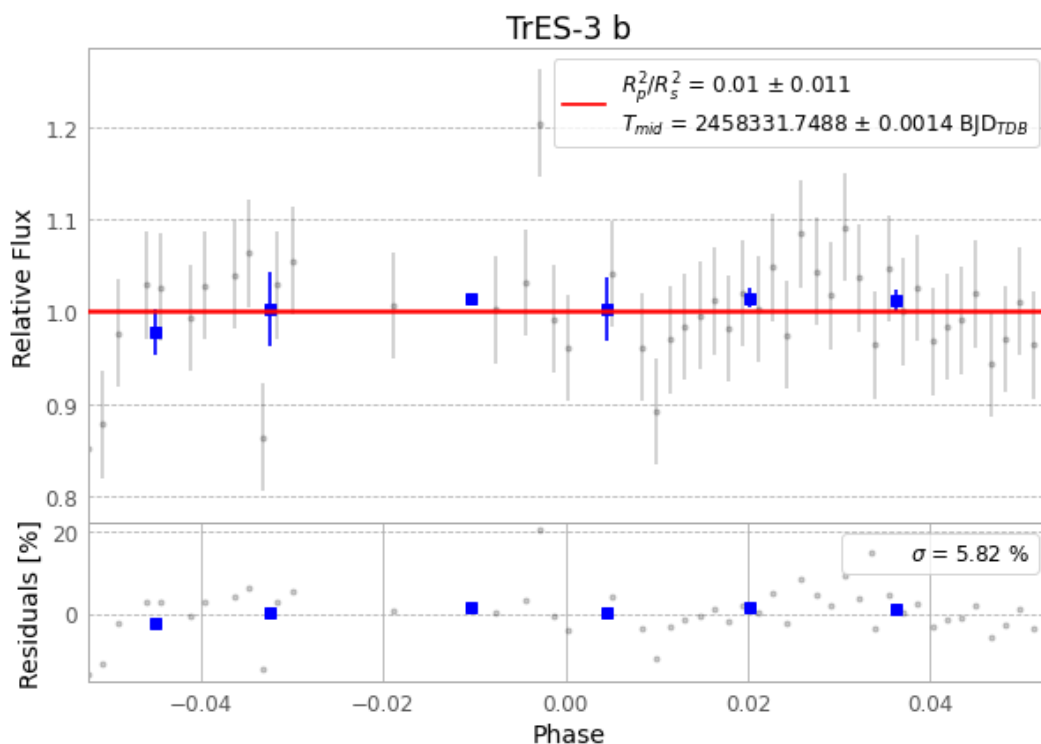
Figure 1 — FinalLightCurve_TrES-3 b_2018-07-31.png (SHA-256 7ecdb59f6f3ee400...)
