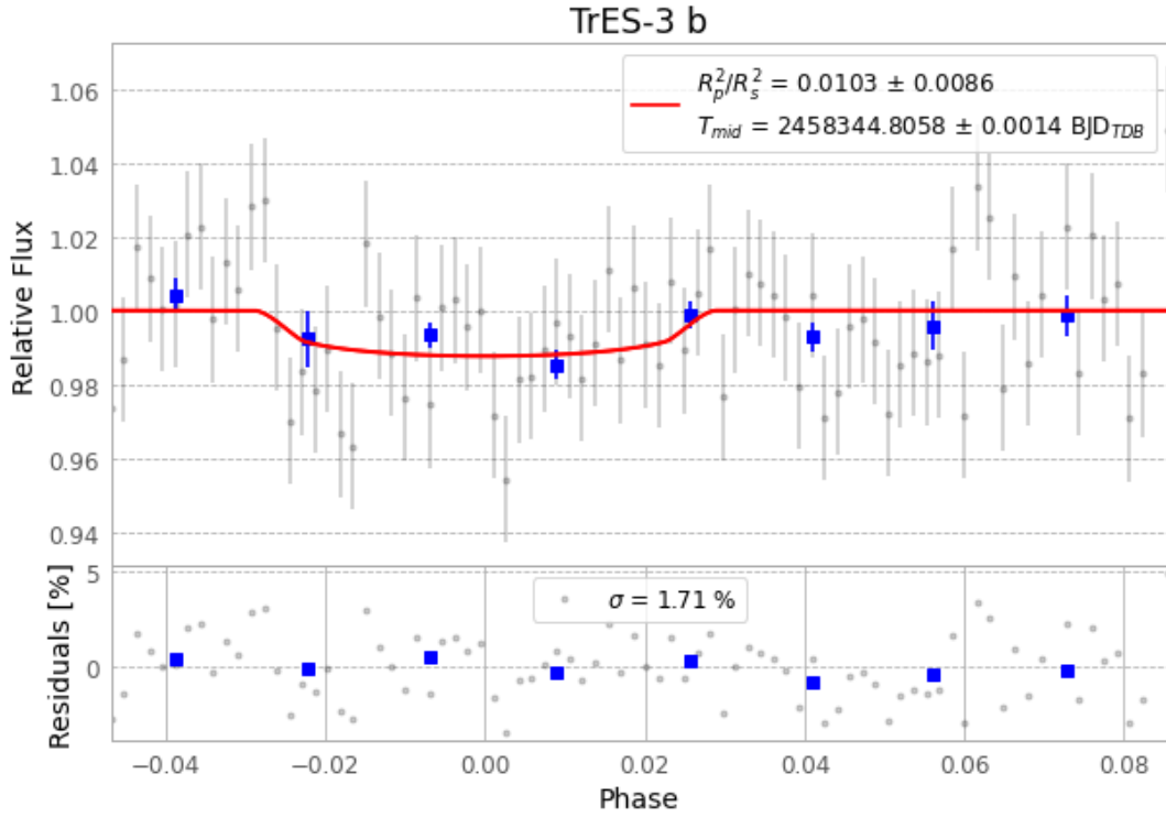
Figure 1 — FinalLightCurve_TrES-3 b_2018-08-13.png (SHA-256 d8cc0d20a149308c...)
