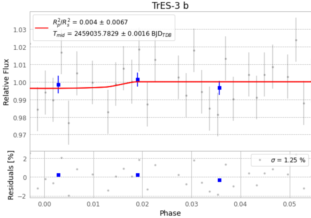
Figure 1 — FinalLightCurve_TrES-3 b_2020-07-04.png (SHA-256 d82eb2fdd4f947c1...)
