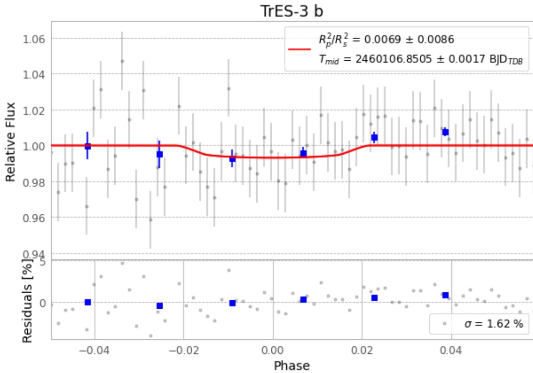
Figure 1 — FinalLightCurve_TrES-3 b_2023-06-10.png (SHA-256 1bb13bcd35d36afa...)
