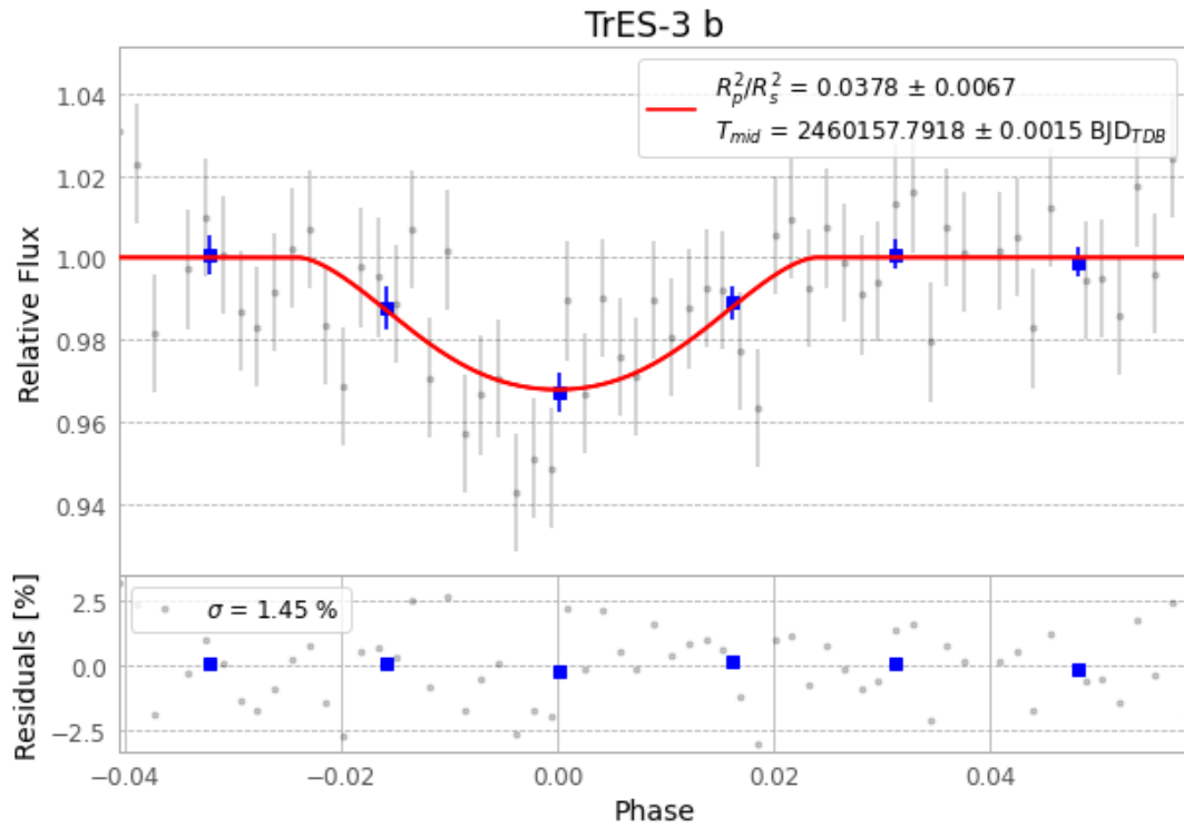
Figure 1 — FinalLightCurve_TrES-3 b_2023-07-31.png (SHA-256 6928d458b4f60298...)
