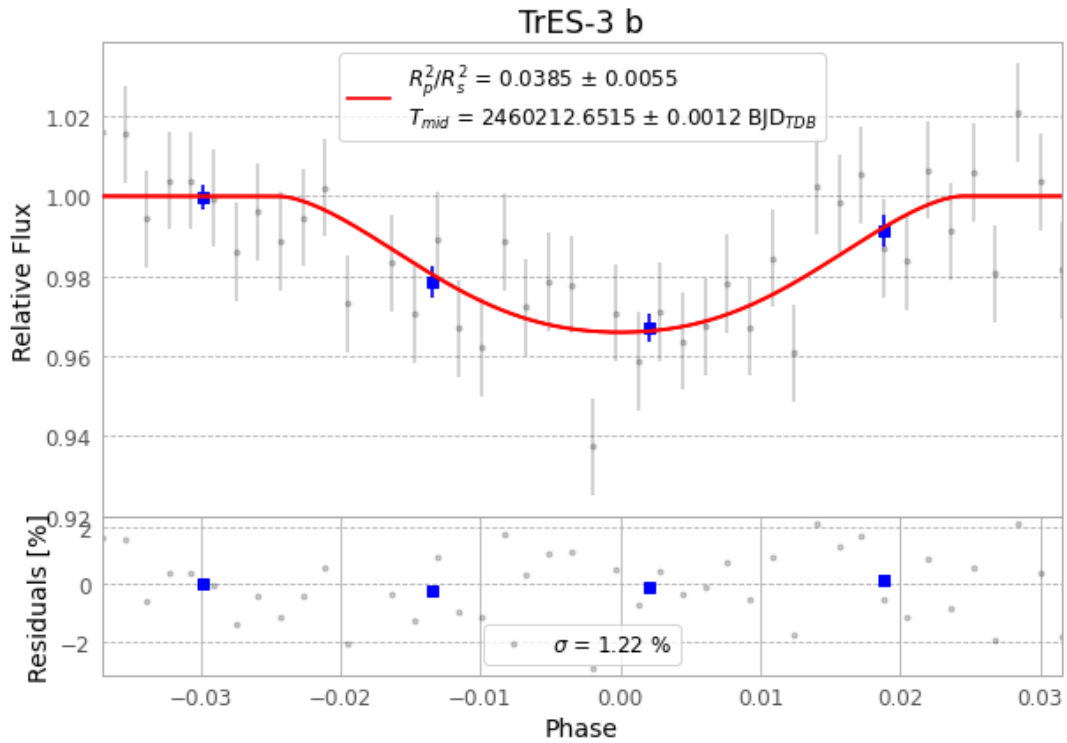
Figure 1 — FinalLightCurve_TrES-3 b_2023-09-24.png (SHA-256 8d10a14b046df189...)
