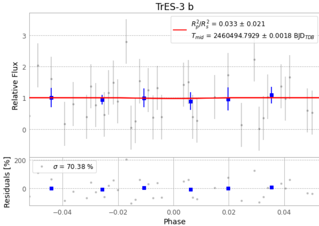
Figure 1 — FinalLightCurve_TrES-3 b_2024-07-02.png (SHA-256 5ac0080a5d7f2b97...)
