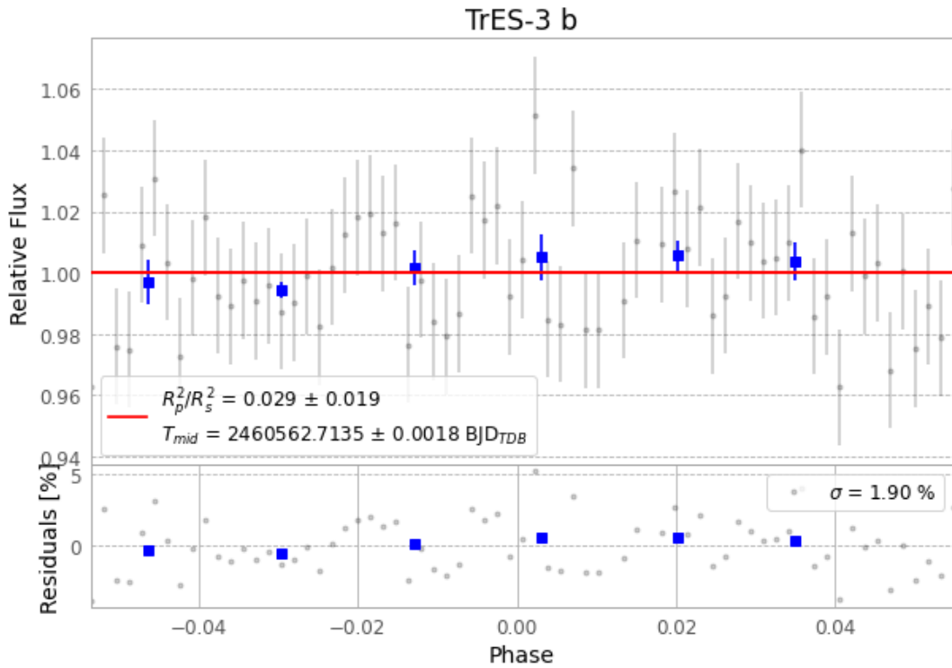
Figure 1 — FinalLightCurve_TrES-3 b_2024-09-08.png (SHA-256 717d7dce99809079...)
