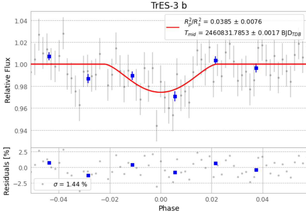
Figure 1 — FinalLightCurve_TrES-3 b_2025-06-04.png (SHA-256 9f76c387f3e94850...)
