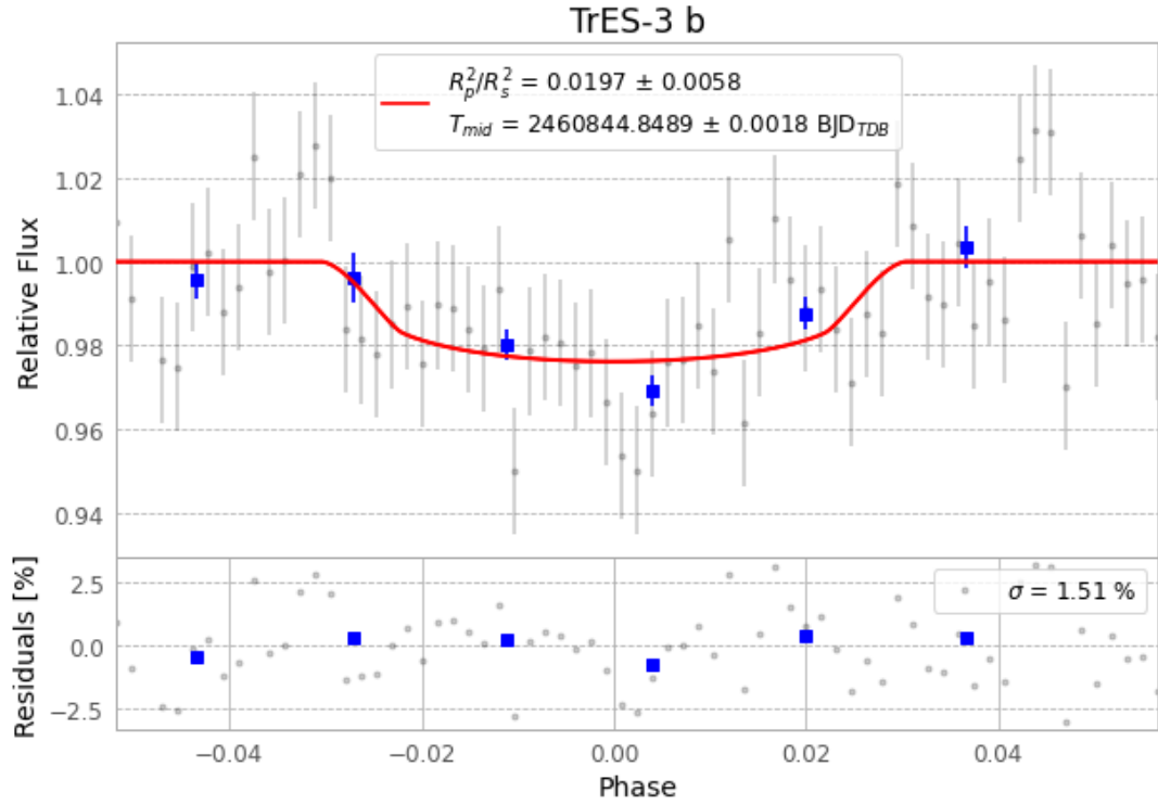
Figure 1 — FinalLightCurve_TrES-3 b_2025-06-17.png (SHA-256 7a90402c3b9de620...)
