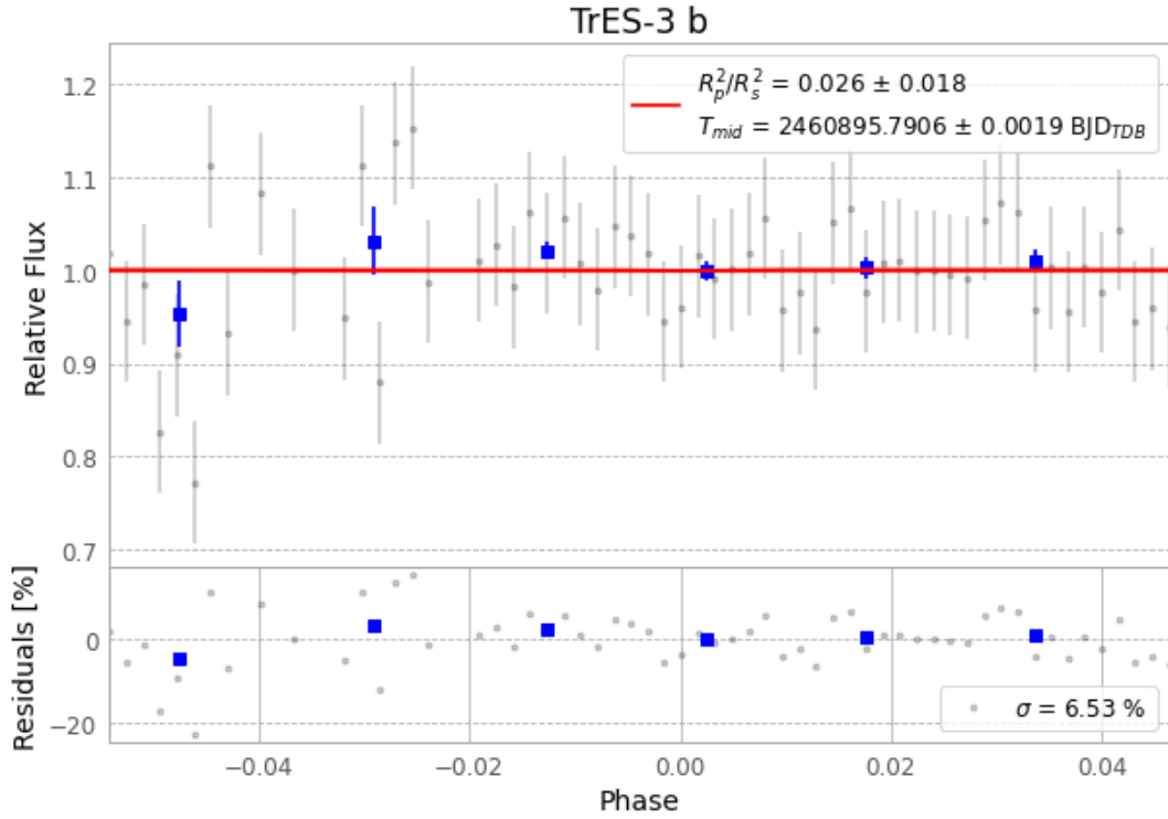
Figure 1 — FinalLightCurve_TrES-3 b_2025-08-07.png (SHA-256 dfde4576730c2bb4...)
