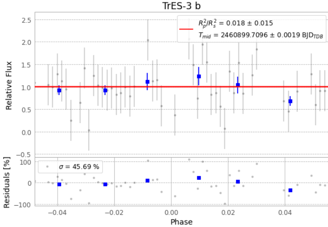
Figure 1 — FinalLightCurve_TrES-3 b_2025-08-11.png (SHA-256 6bf1c1d5707e3898...)
