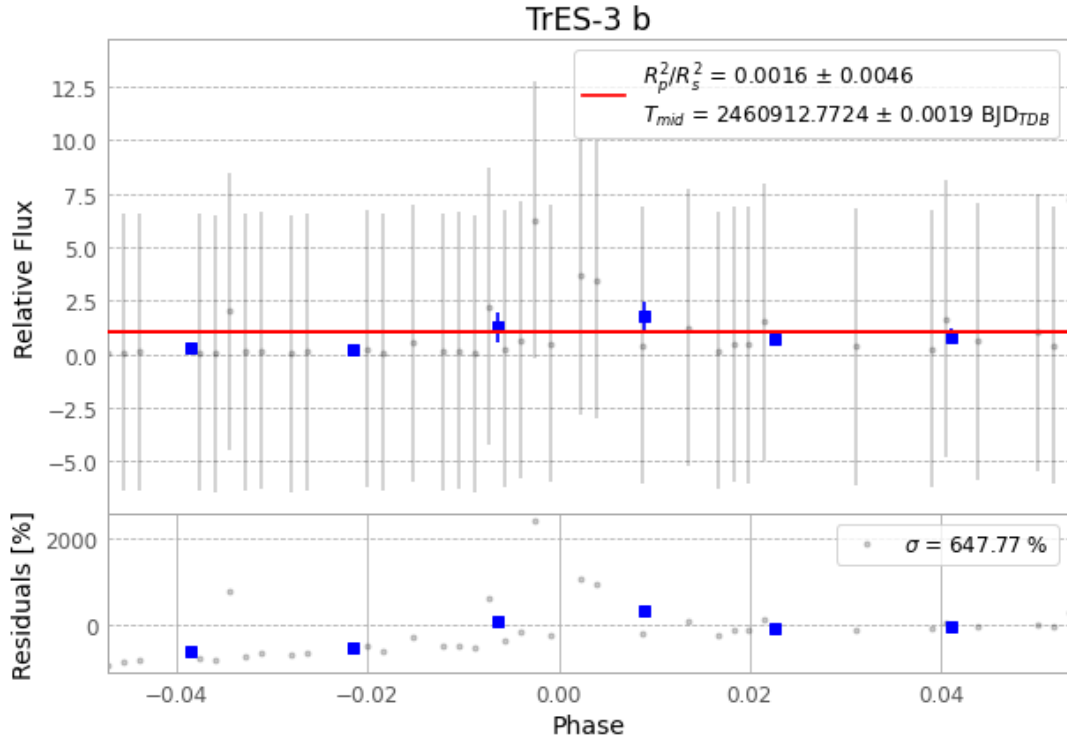
Figure 1 — FinalLightCurve_TrES-3 b_2025-08-24.png (SHA-256 35897815099a81cf...)
