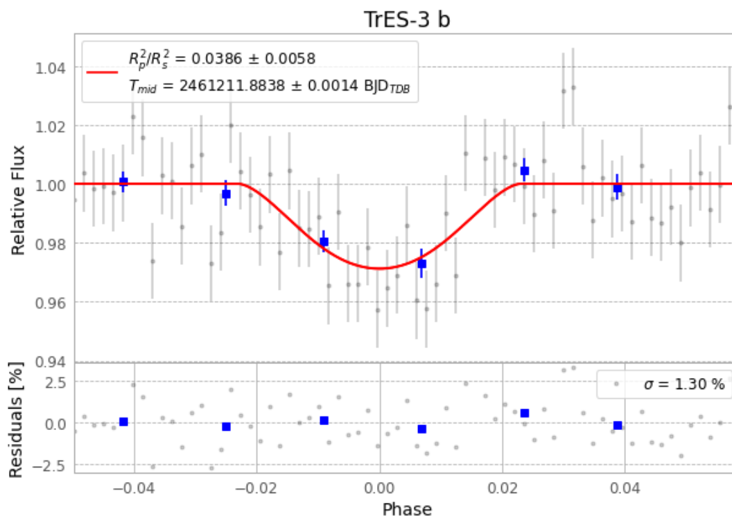
Figure 1 — FinalLightCurve_TrES-3 b_2026-06-20.png (SHA-256 61f336c056653d71...)
