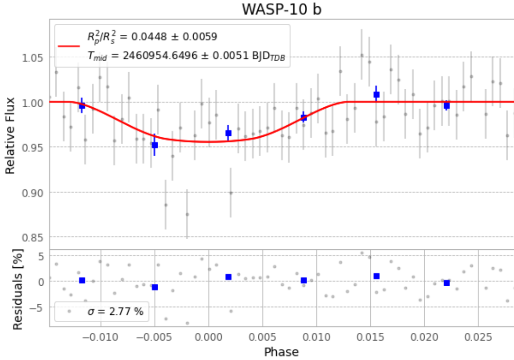
Figure 1 — FinalLightCurve_WASP-10 b_2025-10-05.png (SHA-256 66899bc3ae9f79a0...)
