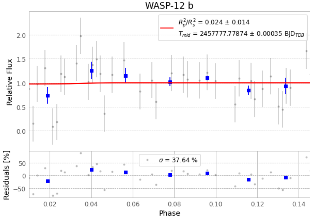
Figure 1 — FinalLightCurve_WASP-12 b_2017-01-23.png (SHA-256 595a9ec87136ce1b...)
