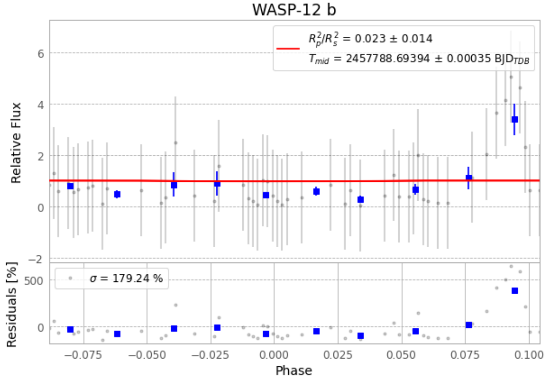
Figure 1 — FinalLightCurve_WASP-12 b_2017-02-03.png (SHA-256 211f81114160c620...)
