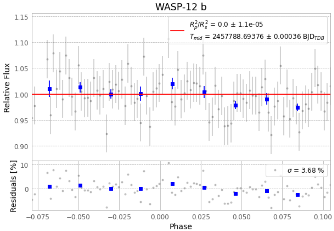
Figure 1 — FinalLightCurve_WASP-12 b_2017-02-03.png (SHA-256 ed722316af9e3a0b...)
