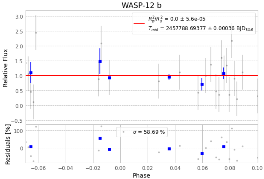
Figure 1 — FinalLightCurve_WASP-12 b_2017-02-03.png (SHA-256 1abb875faf4afdc8...)
