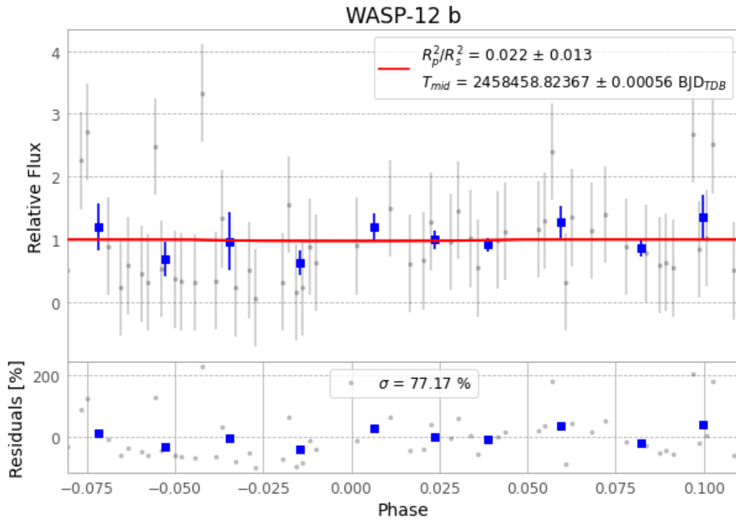
Figure 1 — FinalLightCurve_WASP-12 b_2018-12-05.png (SHA-256 897c3a9c441cc1c6...)
