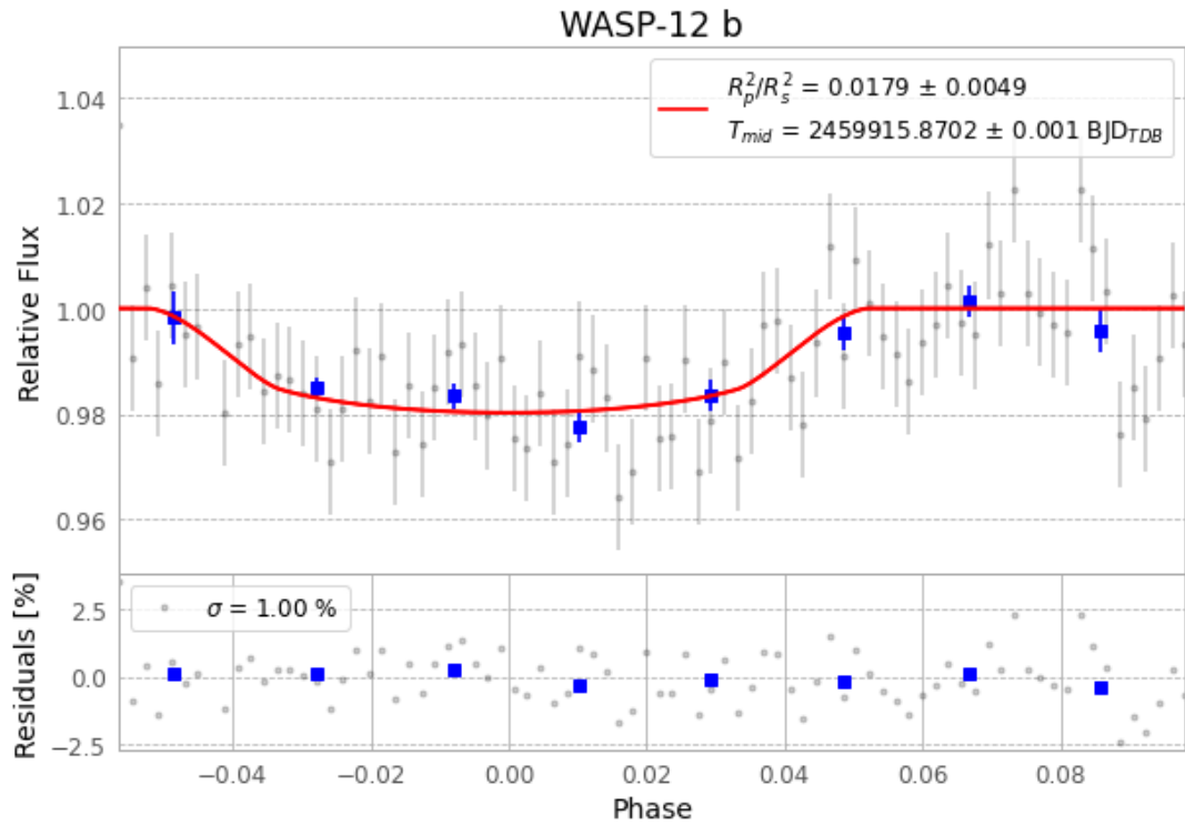
Figure 1 — FinalLightCurve_WASP-12 b_2022-12-02.png (SHA-256 c95d90d12d4e98db...)
